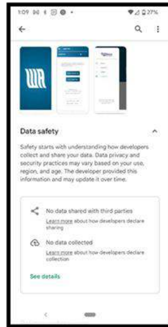
Figure 2: Android App
