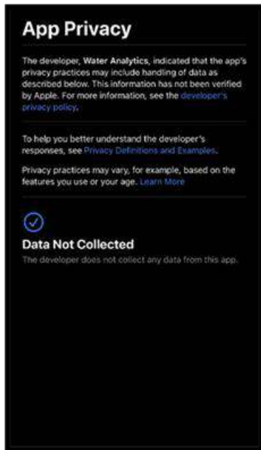
Figure 1: iOS App
