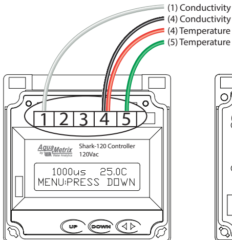
Shark-120 Controller
